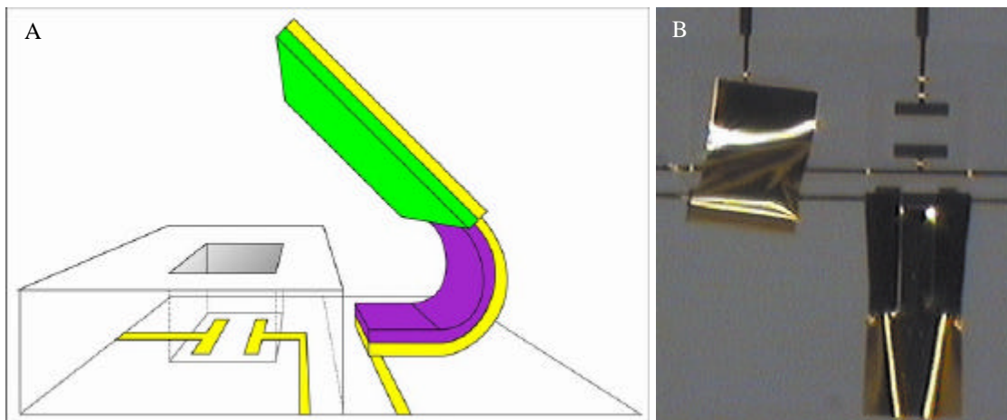
Colour Plate 13.3. Cell clinics: schematic picture (A), closed and open.
