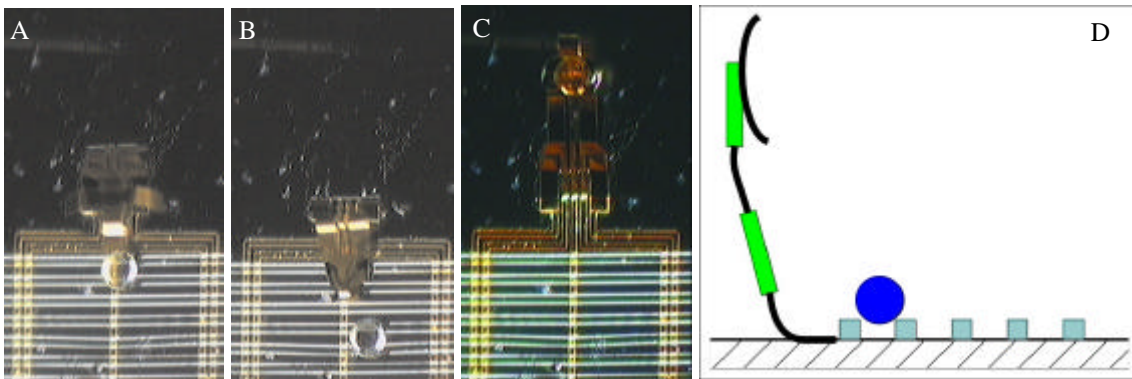
Colour Plate 13.2. A microrobot arm made of PPy microactuators.
