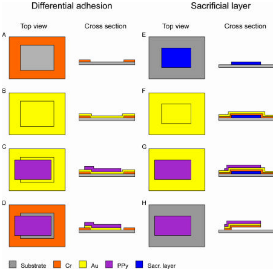
Colour Plate 13.1. A sketch of the fabrication schemes for the differential adhesion method.
